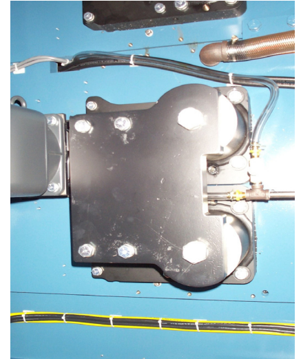
Brushless Motor Upgrade shown with Outboard Cylinder Stiffener Upgrade (7993671)
